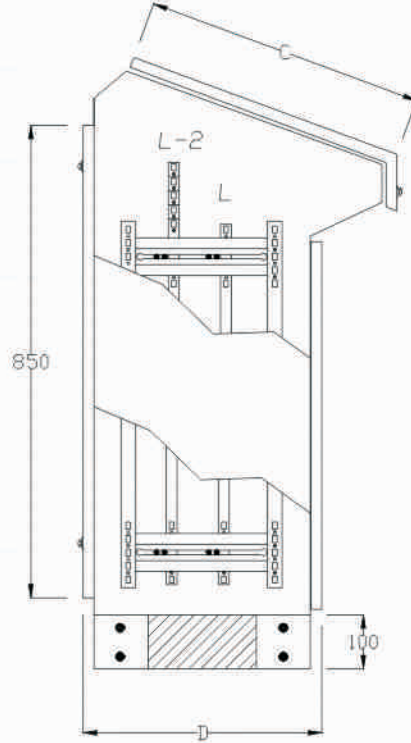
MONTAJ PLAKASI MOUNTING PLATE
